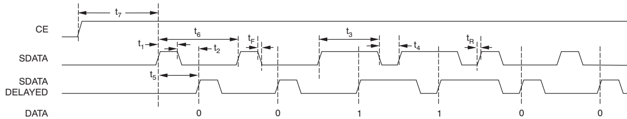
Figure 2. SDATA/CE Timing
